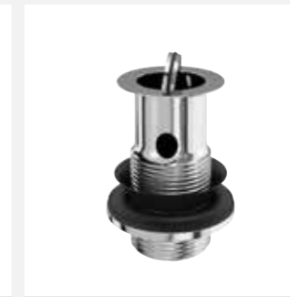
Flip-top basin waste slotted D: 61, W: 61, H: 71 For use with baths with an overflow Code: W18 Price: £22
